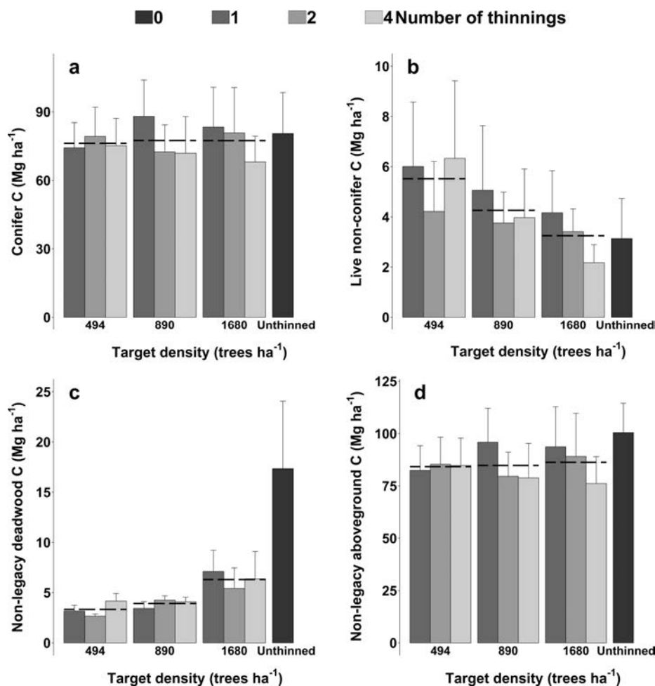
Fig. 2. Effects of thinning treatment on the three C pools predicted to be affected by treatment. (a) live conifers, (b) live non-conifers, (c) non-legacy deadwood. The final panel (d) is the sum of the three previous three pools. The bars are grouped by target density, shown on the x-axis. Within each density level three different thinning regimes (1, 2 or 4 entries) were used to achieve the target density (Table 2). The dashed lines across the three grouped bars are the average of all number-of-entry treatments within a density and represent the main effect of density on C stores. Error bars represent one standard error of the mean.
