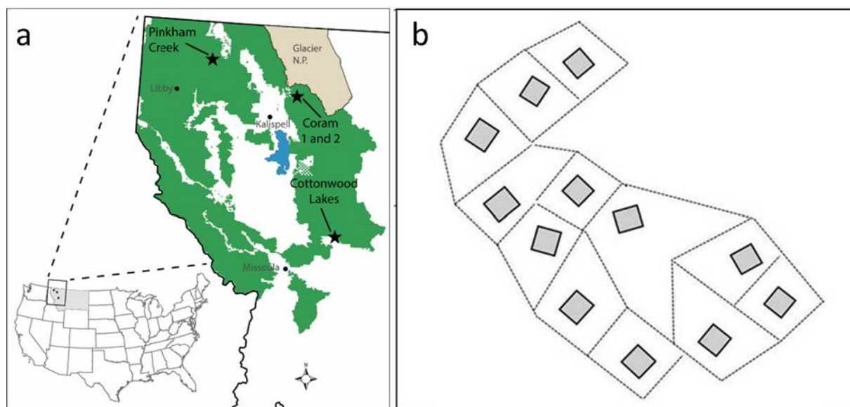
Fig. 1. (a). Locations of the four study sites (i.e. blocks) of the Western Larch Density Management Study in the northwest Montana, USA. (b). An example layout of the plots within a site. Gray squares are the 0.04 ha treatment plots (i.e., experimental units) and the white polygons demarcated by the dashed lines are buffer zones thinned with the same treatment.
